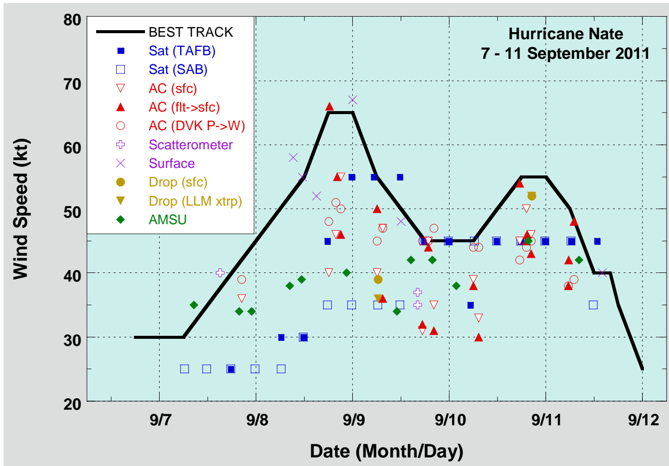
Figure 2. Selected wind observations and best track maximum sustained surface wind speed curve for Hurricane Nate, 7-11 September, 2011. Aircraft observations have been adjusted for elevation using 90%, 80%, and 80% adjustment factors for observations from 700 mb, 850 mb, and 1500 ft, respectively. Dropwindsonde observations include actual 10 m winds (sfc), as well as surface estimates derived from the mean wind over the lowest 150 m of the wind sounding (LLM). Advanced Dvorak Technique estimates represent linear averages over a three-hour period centered on the nominal observation time. AMSU intensity estimates are from the Cooperative Institute for Meteorological Satellite Studies technique. Dashed vertical lines correspond to 0000 UTC.
