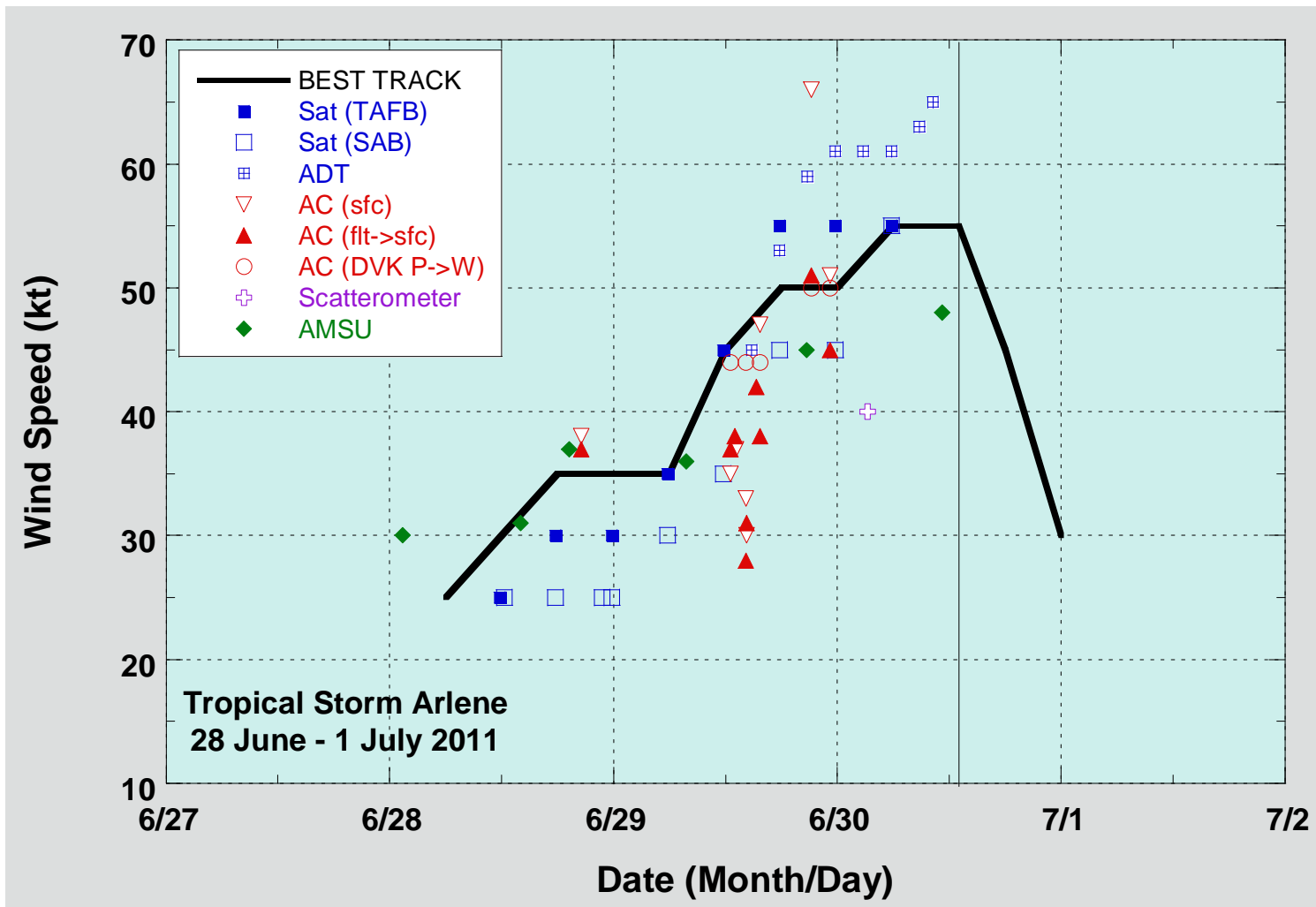
Figure 2. Selected wind observations and best track maximum sustained surface wind speed curve for Tropical Storm Arlene, 28 June – 1 July 2011. Aircraft observations have been adjusted for elevation using 90%, 80%, and 80% adjustment factors for observations from 700 mb, 850 mb, and 1500 ft, respectively. Advanced Dvorak Technique estimates represent linear averages over a three-hour period centered on the nominal observation time. AMSU intensity estimates are from the Cooperative Institute for Meteorological Satellite Studies technique. Dashed vertical lines correspond to 0000 UTC. Solid vertical black line denotes landfall.
