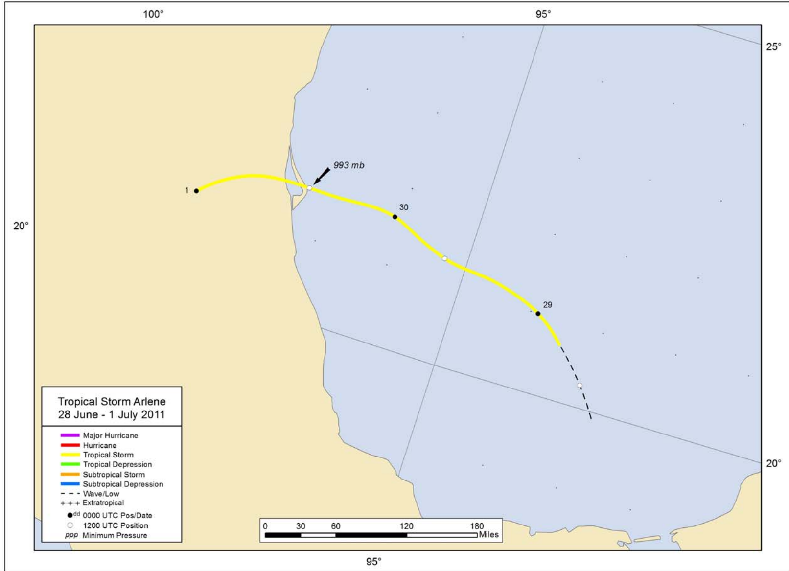
Figure 1. Best track positions for Tropical Storm Arlene, 28 June – 1 July 2011.
